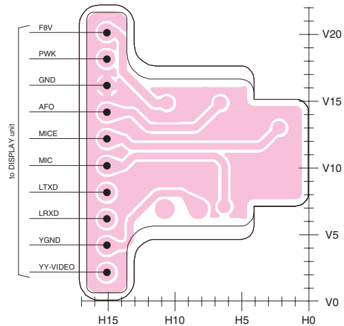
• BOTTOM VIEW (CONNECT UNIT)
